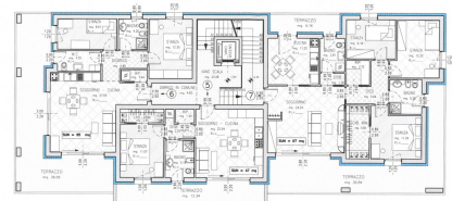
Piano Piano Primo Scale 1:100
